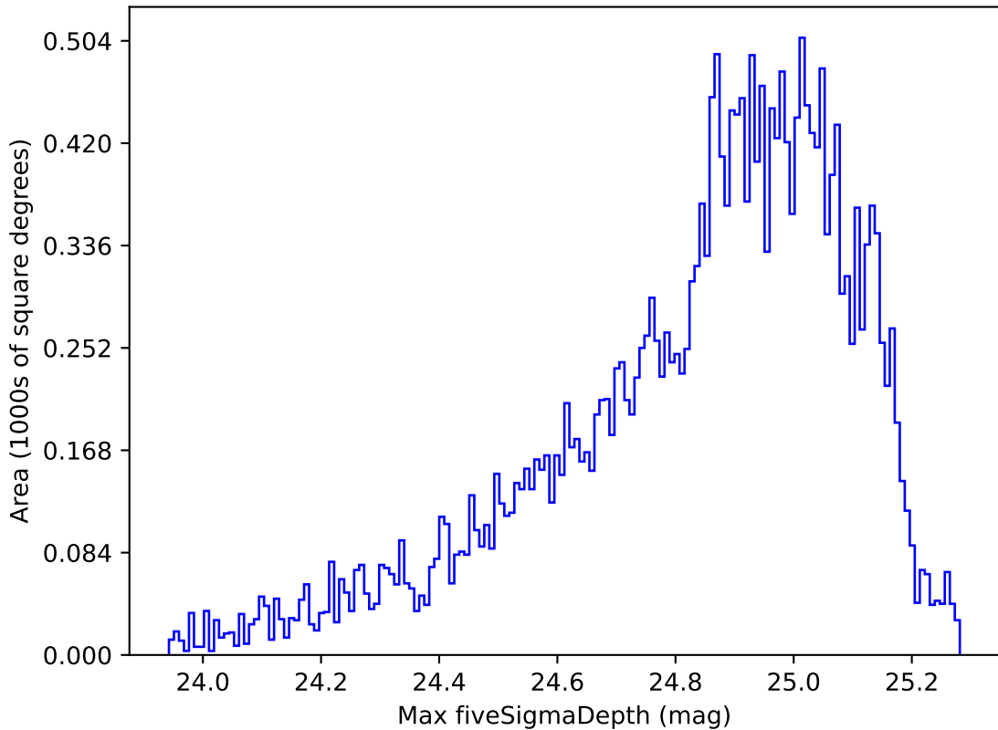
ddf_acor_sf20_lsf0_lsr0_v3.4_10yrs Yr 1 g band: Max fiveSigmaDepth
