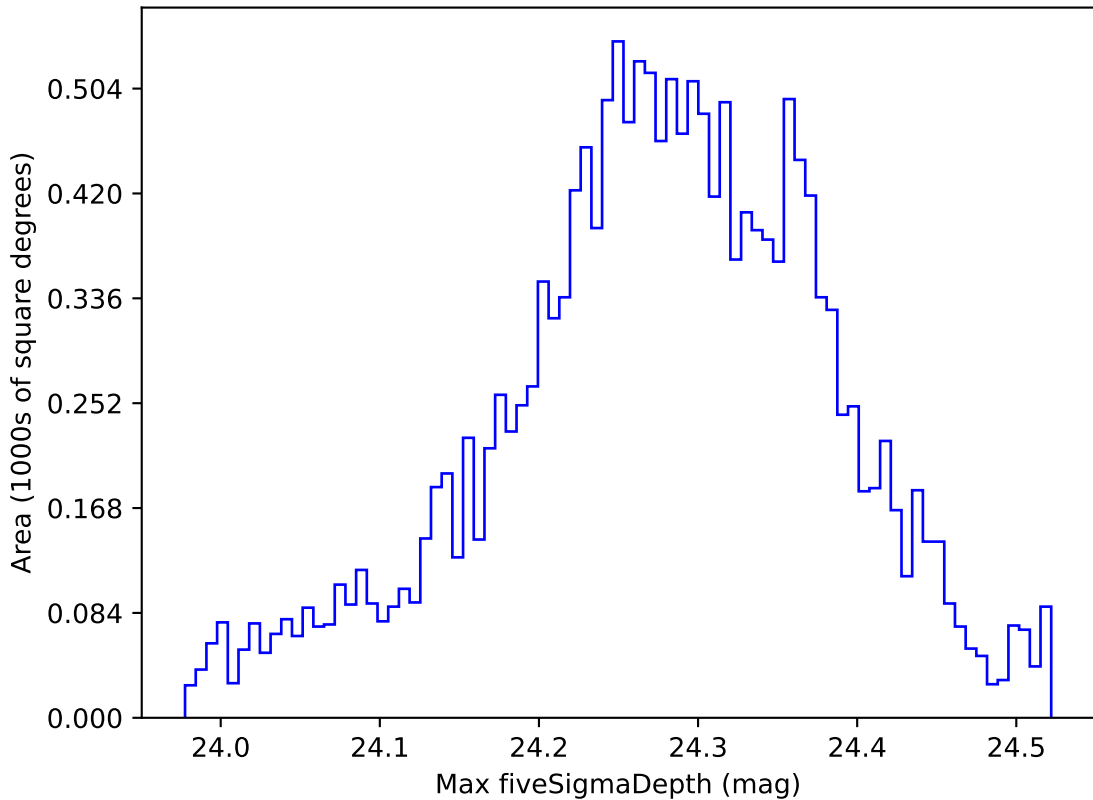
ddf_acor_sf20_lsf0_lsr0_v3.4_10yrs WFD i band: Max fiveSigmaDepth
