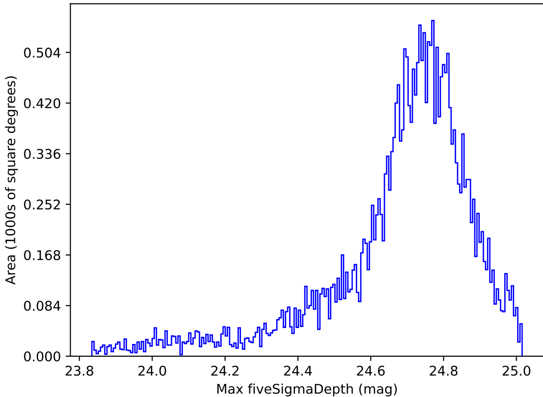
ddf_acor_sf20_lsf0_lsr0_v3.4_10yrs All sky r band: Max fiveSigmaDepth
