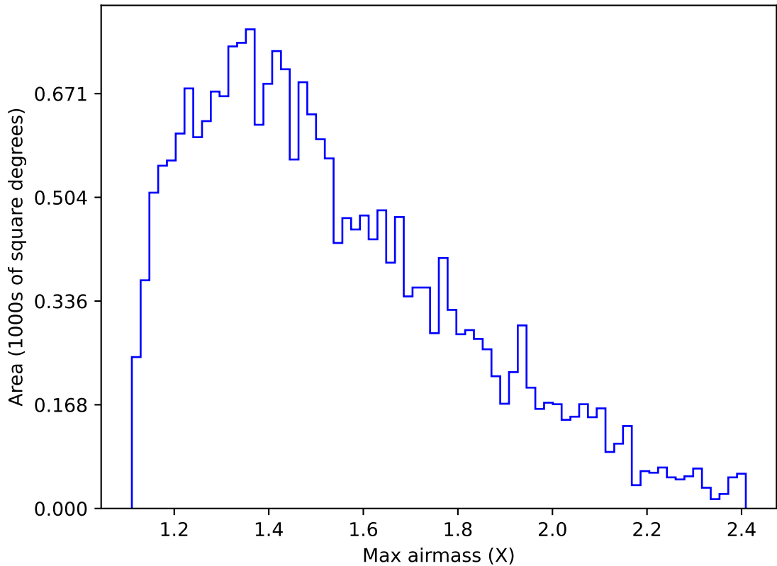
ddf_acor_sf20_lsf0_lsr0_v3.4_10yrs Yr 1 u band: Max airmass
