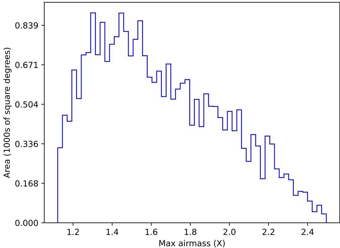
ddf_acor_sf20_lsf0_lsr0_v3.4_10yrs Yr 1 g band: Max airmass
