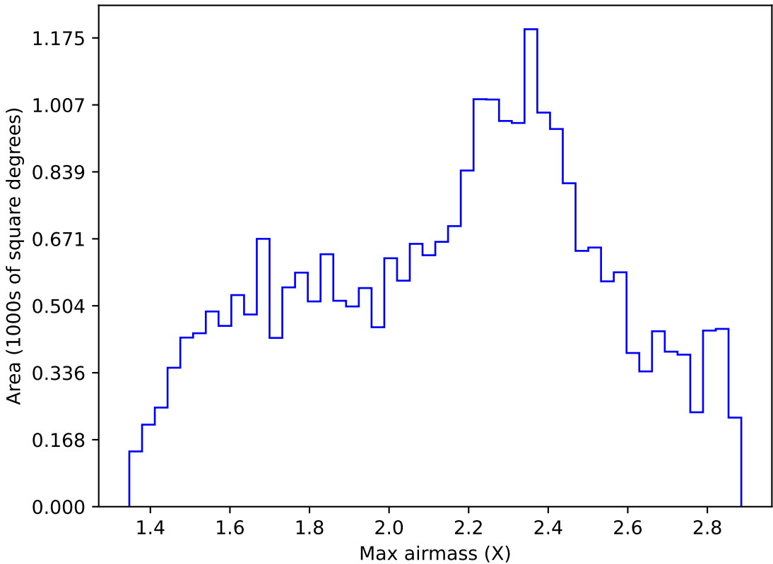
ddf_acor_sf20_lsf0_lsr0_v3.4_10yrs Yr 1 all bands: Max airmass
