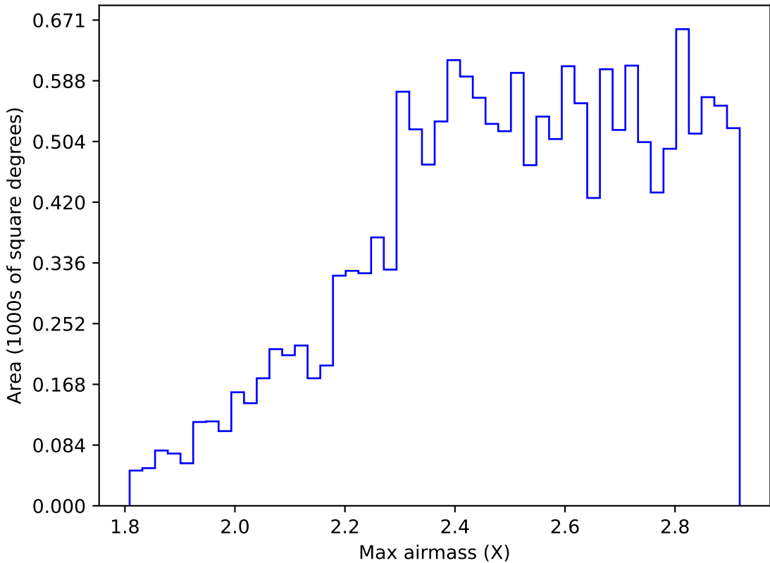
ddf_acor_sf20_lsf0_lsr0_v3.4_10yrs WFD z band: Max airmass
