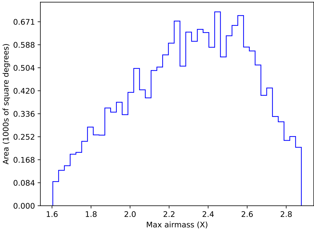
ddf_acor_sf20_lsf0_lsr0_v3.4_10yrs WFD y band: Max airmass
