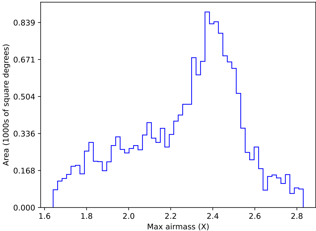
ddf_acor_sf20_lsf0_lsr0_v3.4_10yrs WFD r band: Max airmass
