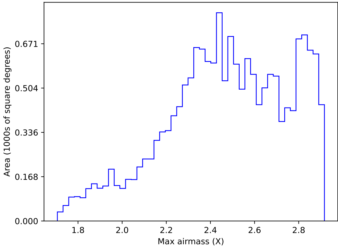
ddf_acor_sf20_lsf0_lsr0_v3.4_10yrs WFD i band: Max airmass
