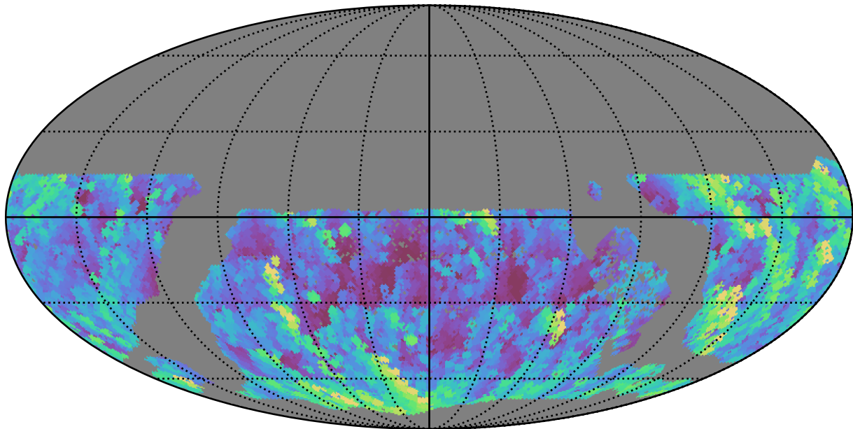
ddf_acor_sf20_lsf0_lsr0_v3.4_10yrs WFD g band: Max airmass
