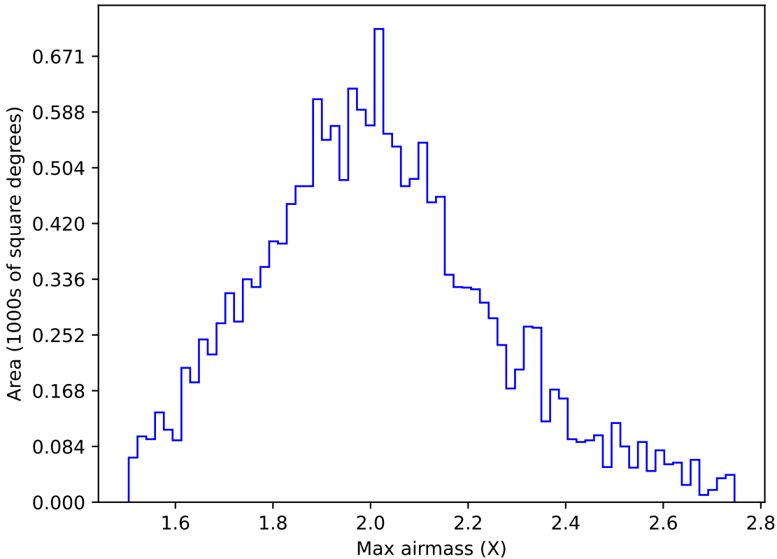
ddf_acor_sf20_lsf0_lsr0_v3.4_10yrs WFD g band: Max airmass
