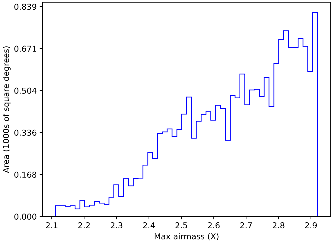
ddf_acor_sf20_lsf0_lsr0_v3.4_10yrs WFD all bands: Max airmass
