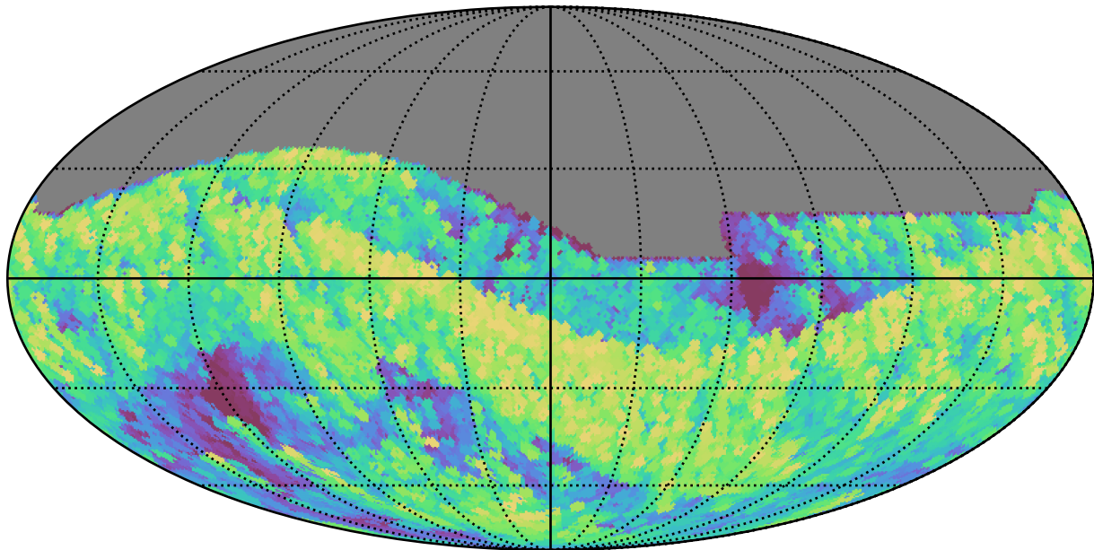
ddf_acor_sf20_lsf0_lsr0_v3.4_10yrs All sky z band: Max airmass
