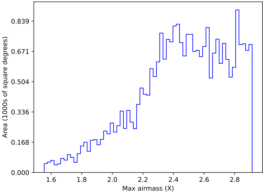
ddf_acor_sf20_lsf0_lsr0_v3.4_10yrs All sky z band: Max airmass
