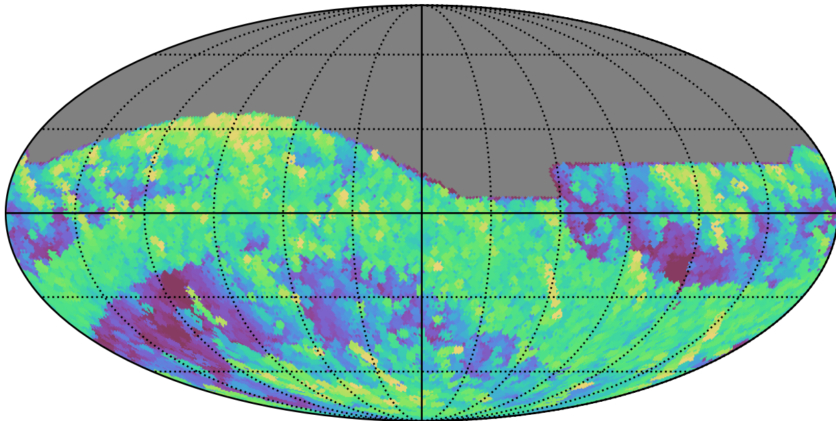
ddf_acor_sf20_lsf0_lsr0_v3.4_10yrs All sky r band: Max airmass
