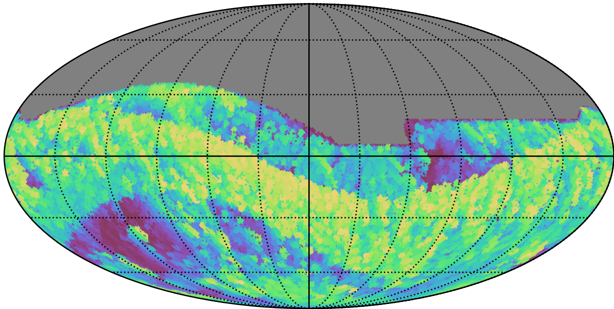
ddf_acor_sf20_lsf0_lsr0_v3.4_10yrs All sky i band: Max airmass
