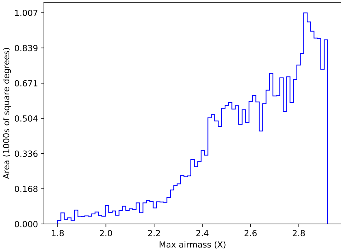
ddf_acor_sf20_lsf0_lsr0_v3.4_10yrs All sky all bands: Max airmass
