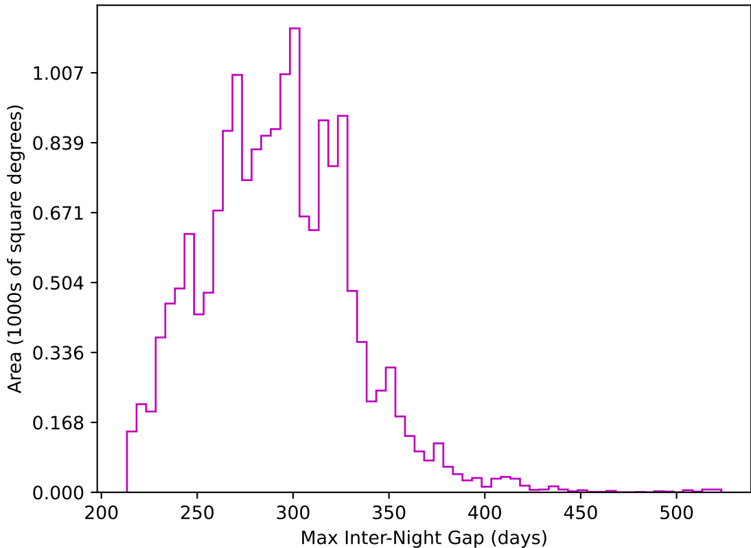
ddf_acor_sf20_lsf0_lsr0_v3.4_10yrs WFD z band: Max Inter-Night Gap
