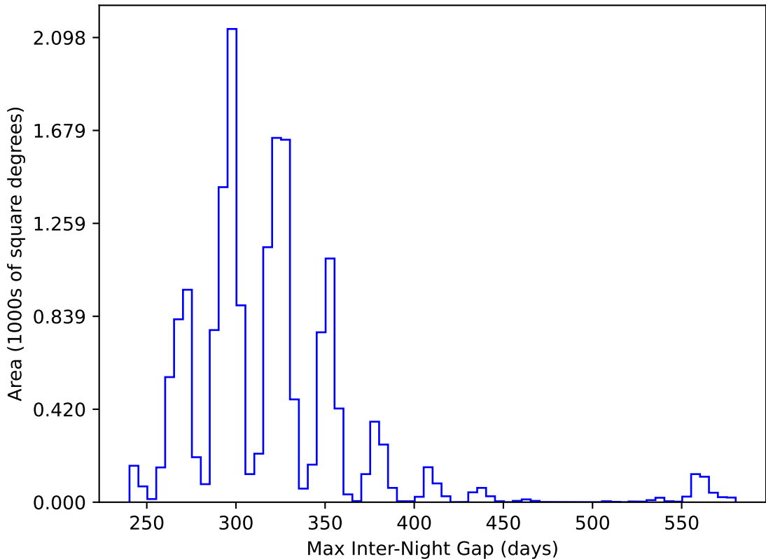
ddf_acor_sf20_lsf0_lsr0_v3.4_10yrs WFD y band: Max Inter-Night Gap
