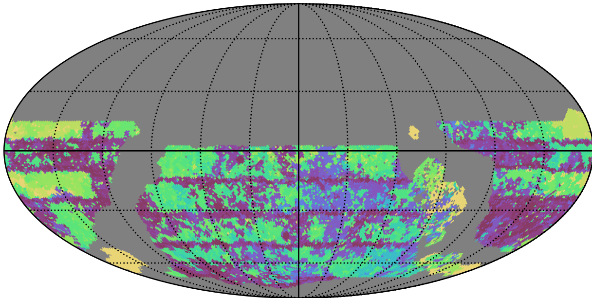
ddf_acor_sf20_lsf0_lsr0_v3.4_10yrs WFD u band: Max Inter-Night Gap
