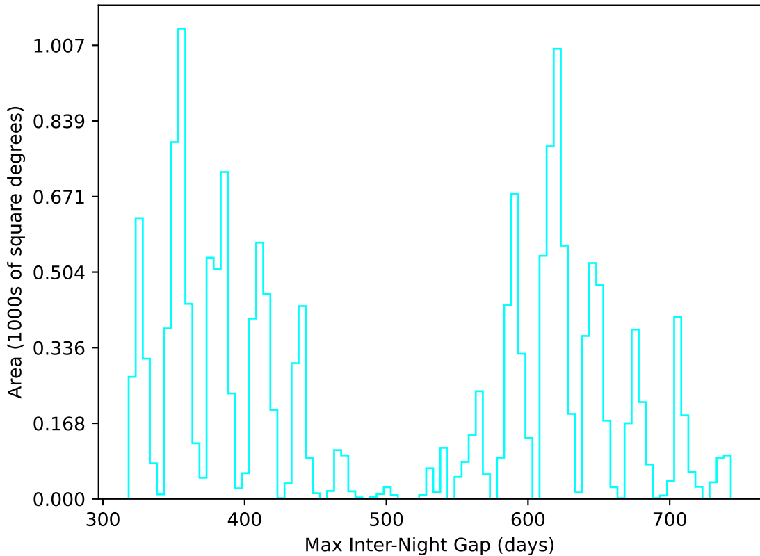
ddf_acor_sf20_lsf0_lsr0_v3.4_10yrs WFD u band: Max Inter-Night Gap
