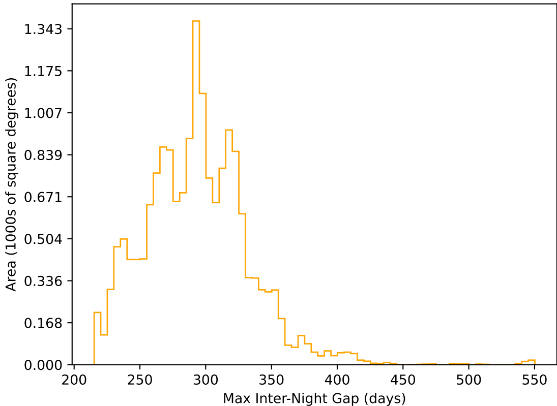
ddf_acor_sf20_lsf0_lsr0_v3.4_10yrs WFD r band: Max Inter-Night Gap
