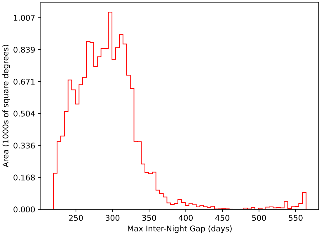
ddf_acor_sf20_lsf0_lsr0_v3.4_10yrs WFD i band: Max Inter-Night Gap
