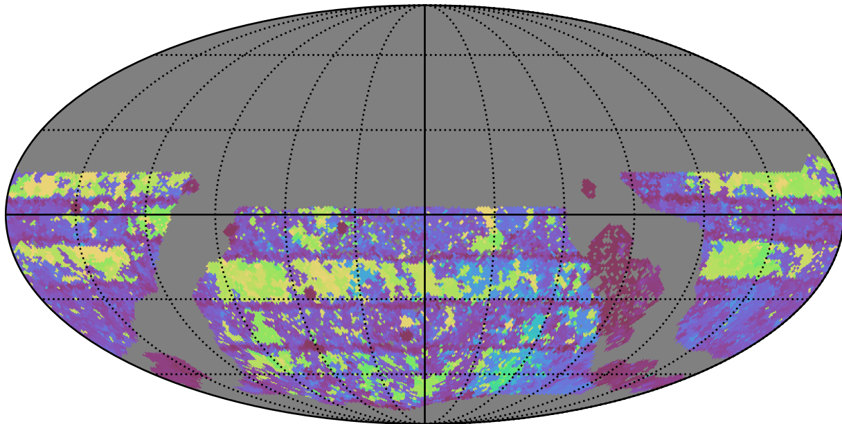
ddf_acor_sf20_lsf0_lsr0_v3.4_10yrs WFD g band: Max Inter-Night Gap
