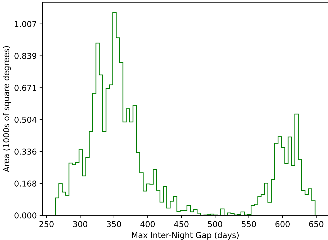
ddf_acor_sf20_lsf0_lsr0_v3.4_10yrs WFD g band: Max Inter-Night Gap
