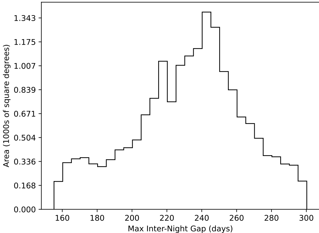
ddf_acor_sf20_lsf0_lsr0_v3.4_10yrs WFD all bands: Max Inter-Night Gap
