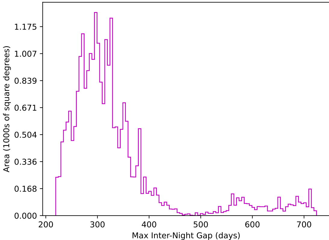
ddf_acor_sf20_ls0_lsr0_v3.4_10yrs All sky z band: Max Inter-Night Gap
