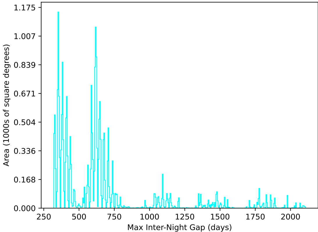
ddf_acor_sf20_ls0_lsr0_v3.4_10yrs All sky u band: Max Inter-Night Gap
