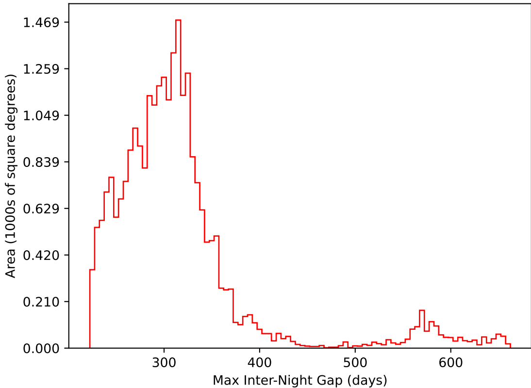
ddf_acor_sf20_lsf0_lsr0_v3.4_10yrs All sky i band: Max Inter-Night Gap
