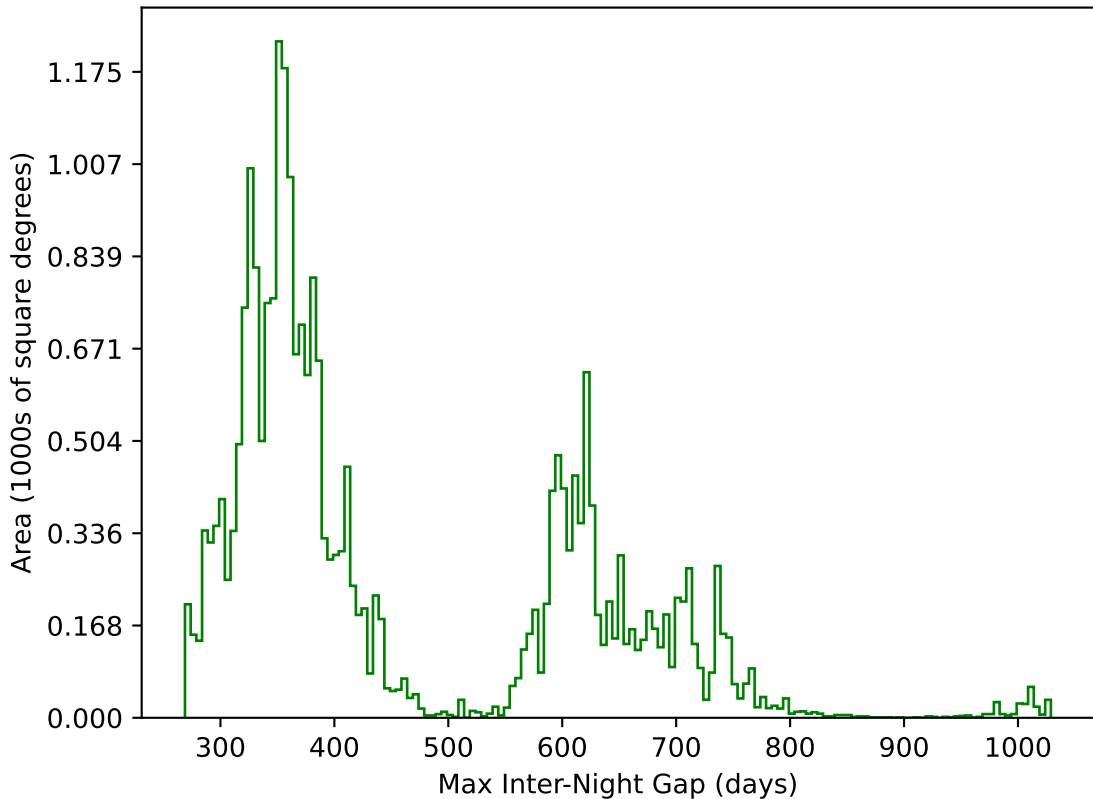
ddf_acor_sf20_ls0_lsr0_v3.4_10yrs All sky g band: Max Inter-Night Gap
