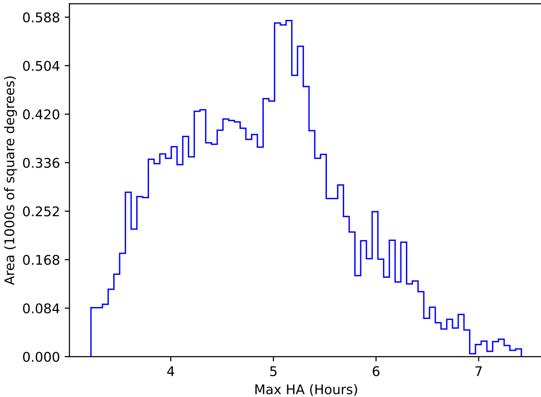
ddf_acor_sf20_lsf0_lsr0_v3.4_10yrs WFD z band: Max HA
