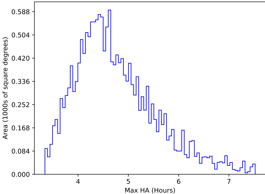
ddf_acor_sf20_lsf0_lsr0_v3.4_10yrs WFD y band: Max HA
