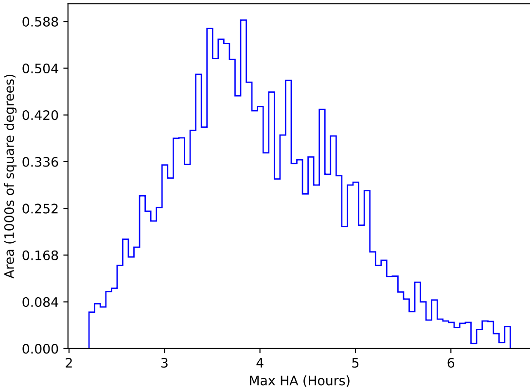
ddf_acor_sf20_lsf0_lsr0_v3.4_10yrs WFD u band: Max HA
