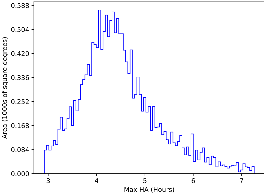
ddf_acor_sf20_lsf0_lsr0_v3.4_10yrs WFD r band: Max HA
