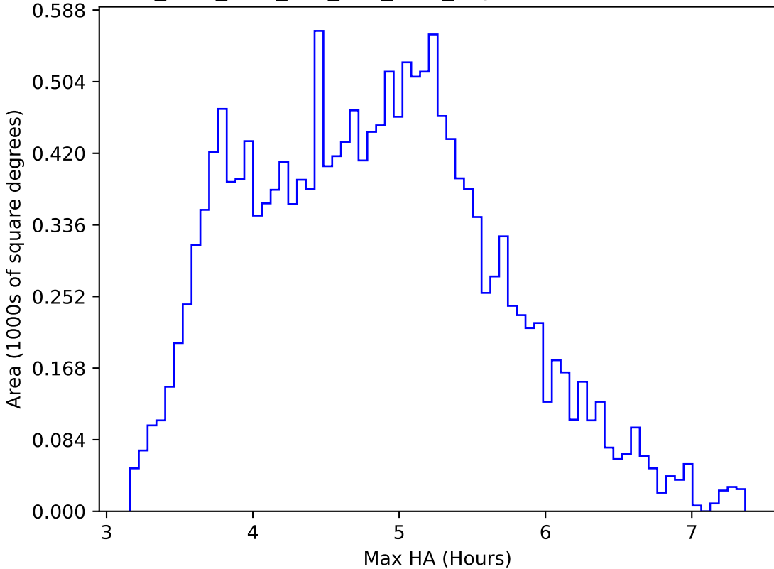
ddf_acor_sf20_ls0_lsr0_v3.4_10yrs WFD i band: Max HA
