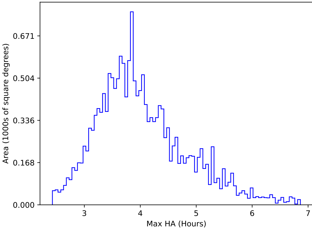
ddf_acor_sf20_ls0_lsr0_v3.4_10yrs WFD g band: Max HA
