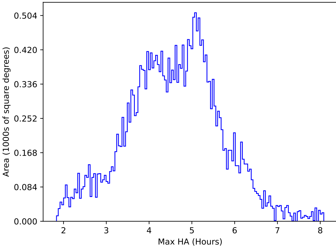
ddf_acor_sf20_lsf0_lsr0_v3.4_10yrs All sky z band: Max HA
