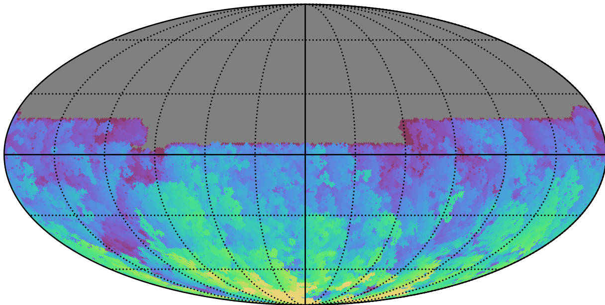
ddf_acor_sf20_lsf0_lsr0_v3.4_10yrs All sky u band: Max HA
