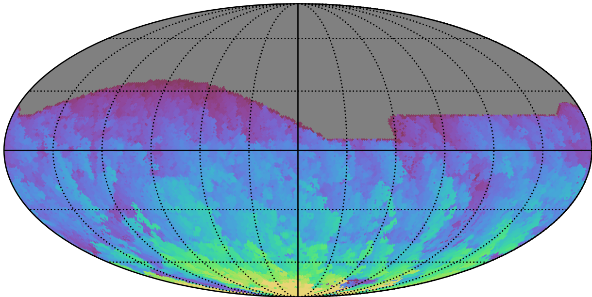
ddf_acor_sf20_lsf0_lsr0_v3.4_10yrs All sky r band: Max HA
