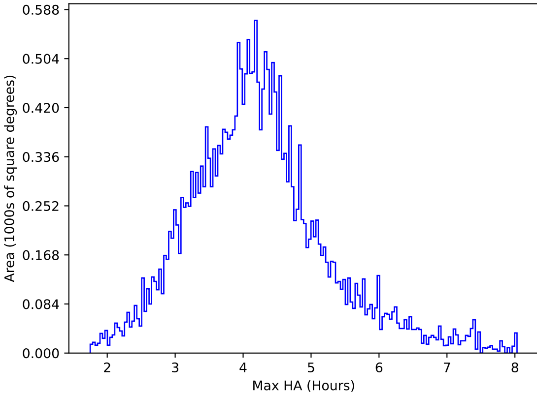
ddf_acor_sf20_lsf0_lsr0_v3.4_10yrs All sky r band: Max HA
