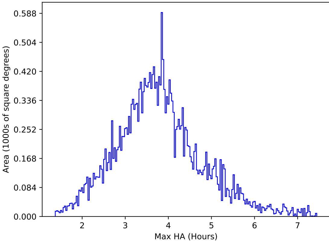
ddf_acor_sf20_lsf0_lsr0_v3.4_10yrs All sky g band: Max HA
