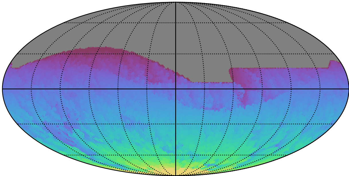
ddf_acor_sf20_lsf0_lsr0_v3.4_10yrs All sky all bands: Max HA
