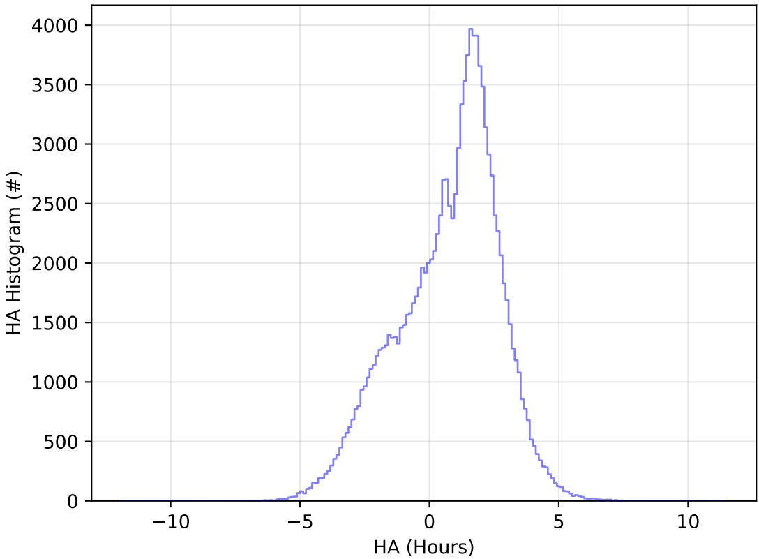
ddf_acor_sf20_lsf0_lsr0_v3.4_10yrs WFD u band: HA Histogram
