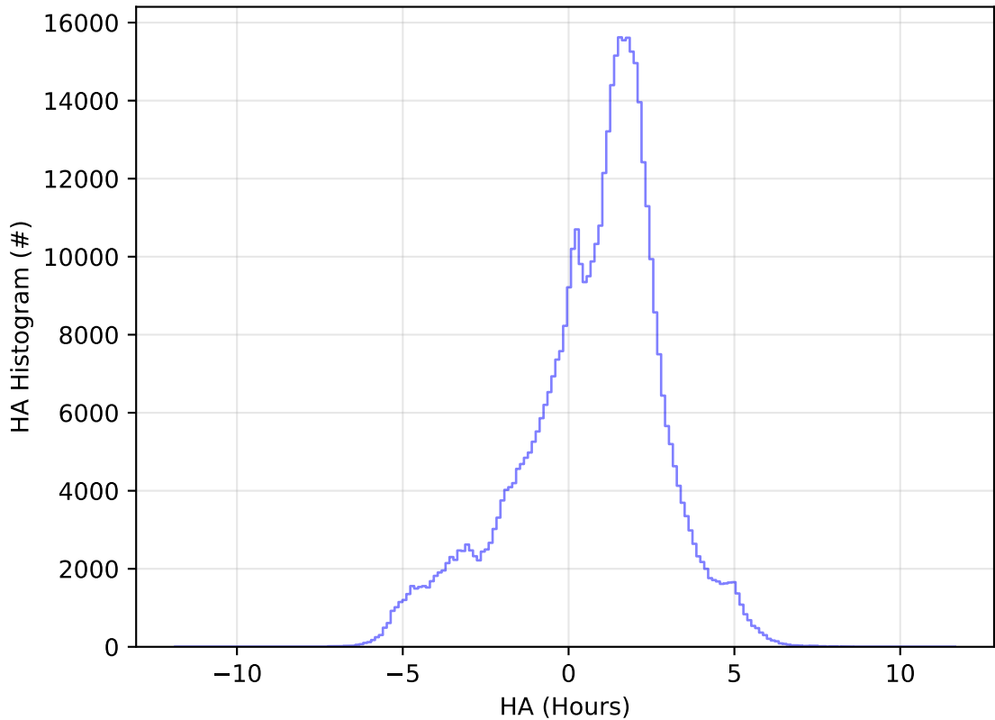
ddf_acor_sf20_lsf0_lsr0_v3.4_10yrs WFD i band: HA Histogram
