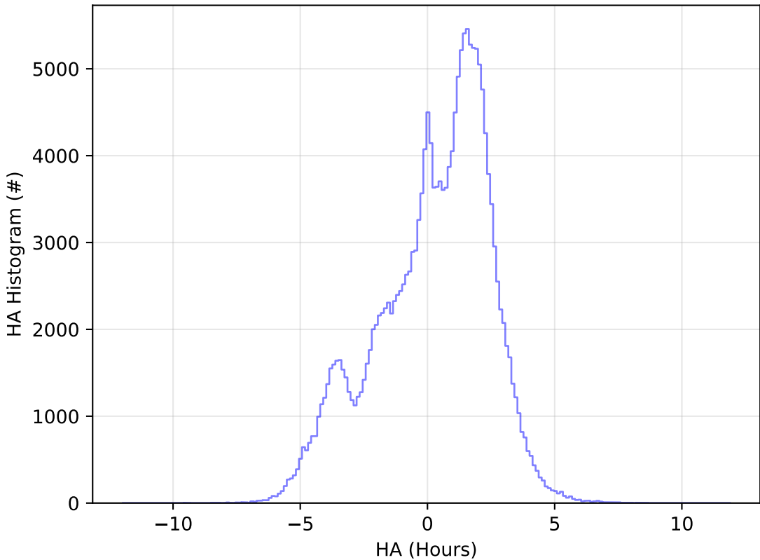
ddf_acor_sf20_lsfl0_lsr0_v3.4_10yrs WFD g band: HA Histogram
