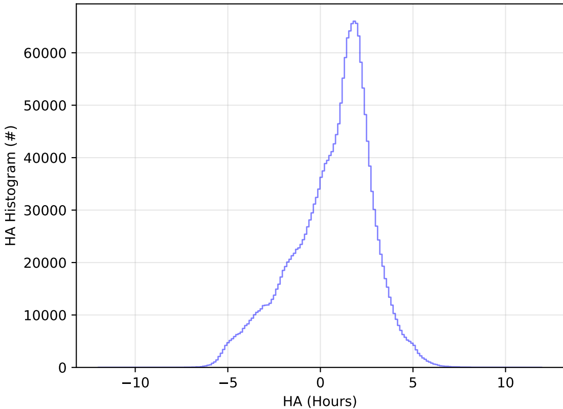
ddf_acor_sf20_lsf0_lsr0_v3.4_10yrs WFD all bands: HA Histogram
