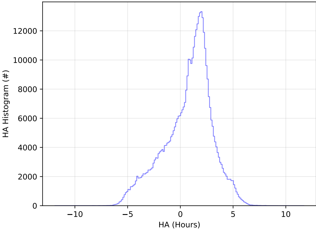
ddf_acor_sf20_lsf0_lsr0_v3.4_10yrs All sky z band: HA Histogram
