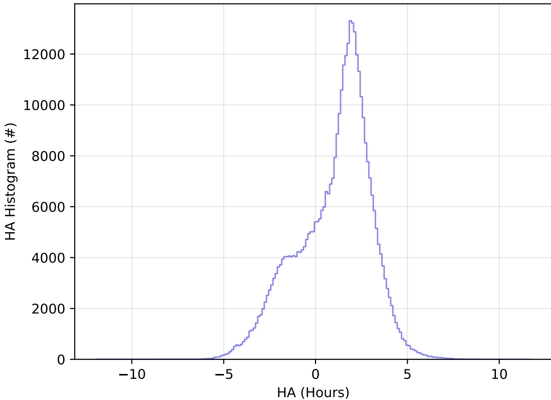
ddf_acor_sf20_lsf0_lsr0_v3.4_10yrs All sky y band: HA Histogram
