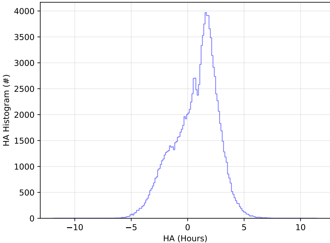
ddf_acor_sf20_lsf0_lsr0_v3.4_10yrs All sky u band: HA Histogram
